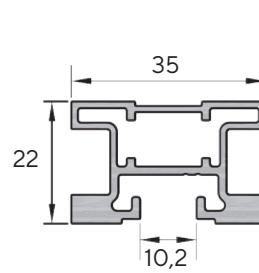
Profil vertical simetric
